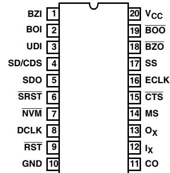
HD-6409 (20 LD PDIP, SOIC) TOP VIEW
